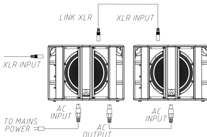
Fig. 8. Parallel connection for S15W cabinets (signal and mains)
