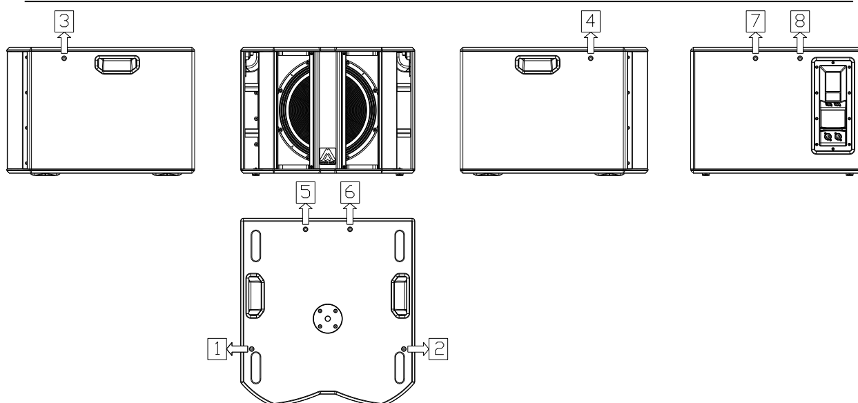
Fig. 10. S15W rigging points
