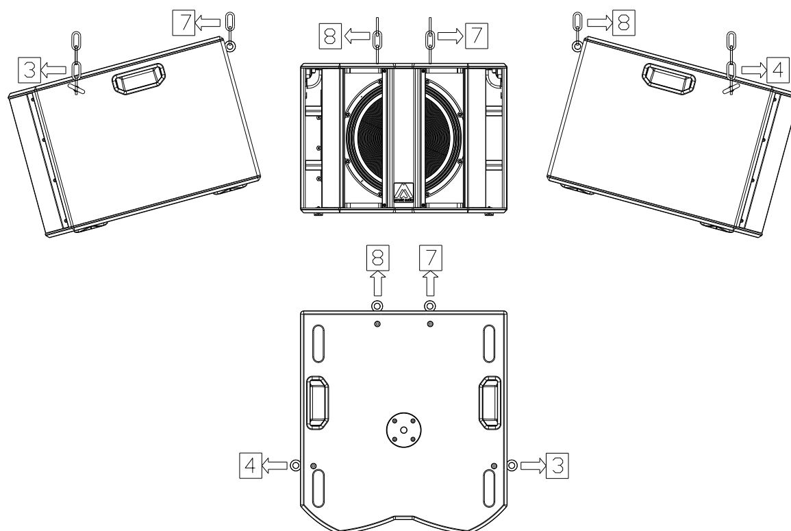
Fig. 12. S15W flying (front points 3&4, back points 7&8)
