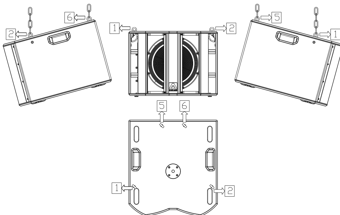
Fig. 11. S15W flying (front points 1&2, back points 5&6)
