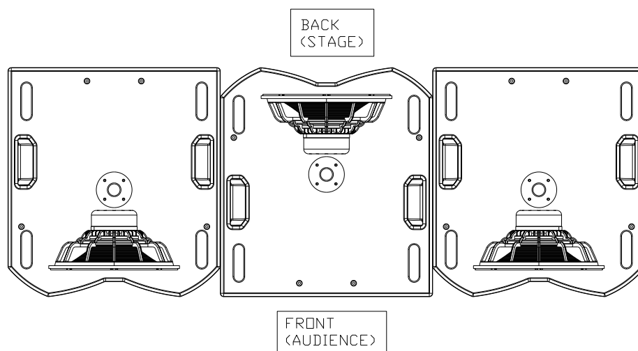
Fig. 4. Cardioid configuration for S15W (horizontal line)
