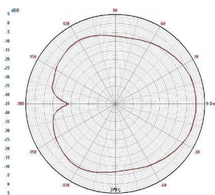
Fig. 9. Cardioid pattern
