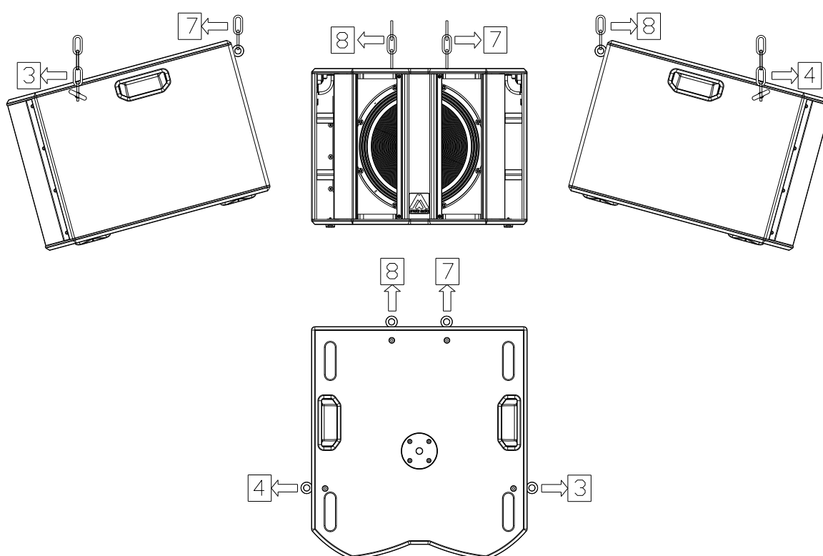
Fig. 7. Flying points 3&4 (front) and 7&8 (back)
