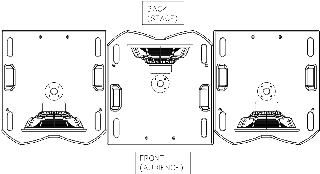
Fig. 11. Cardioid configuration for S15WP (horizontal line)
