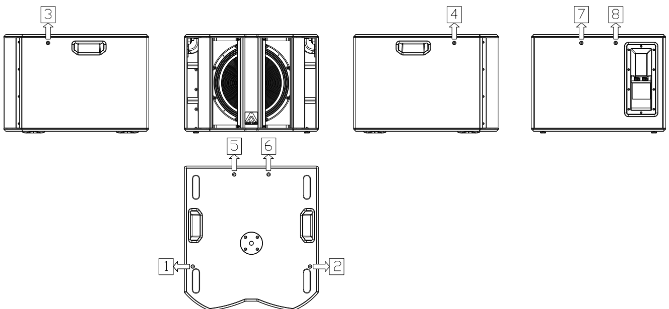
Fig. 5. S15WP M8 rigging points
