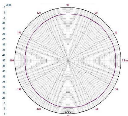
Fig. 8. Traditional polar pattern of a subwoofer at 40Hz
