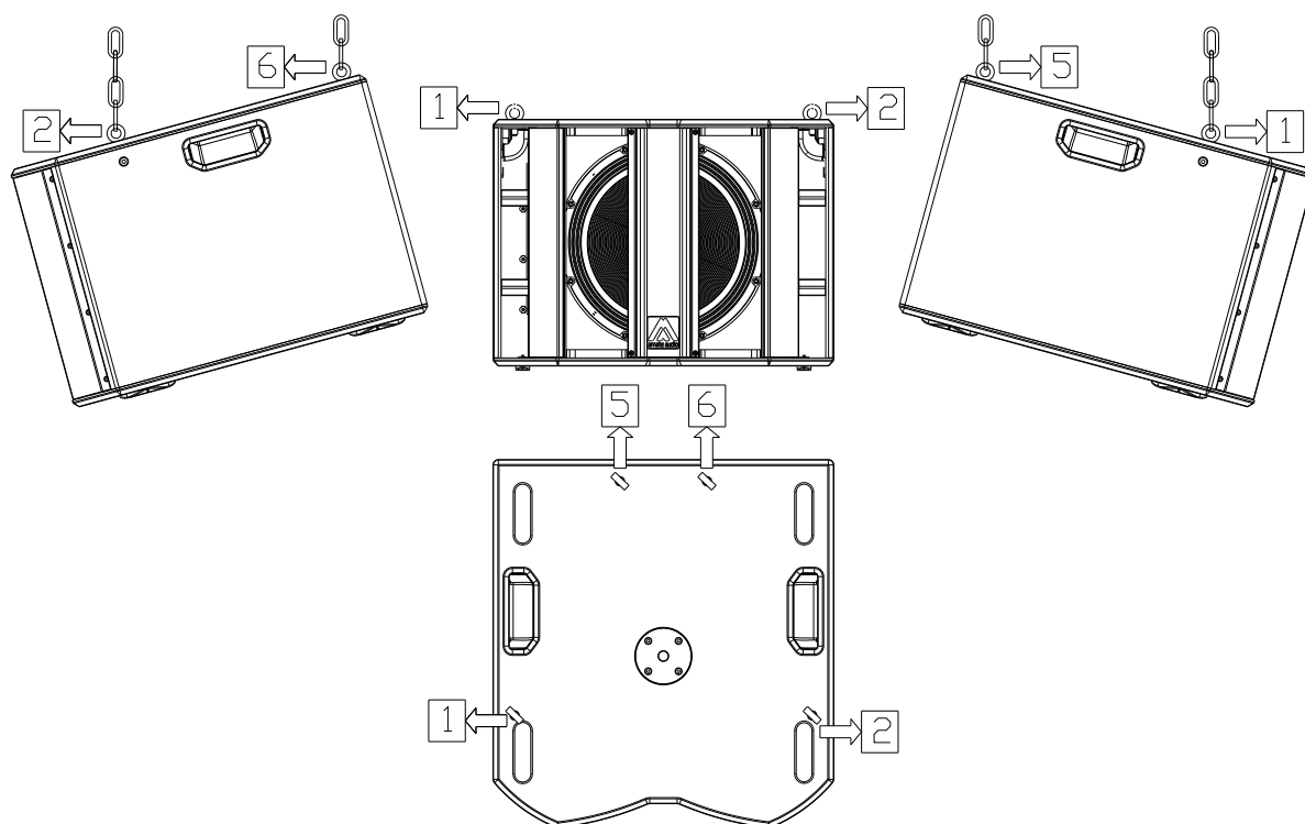
Fig. 6. Flying points 1&2 (front) and 5&6 (back)
