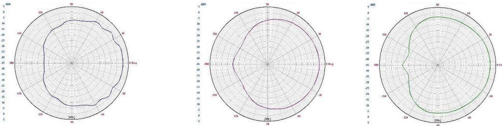
Fig. 13. Back energy rejection at 40 Hz / 50 Hz / 63 Hz
