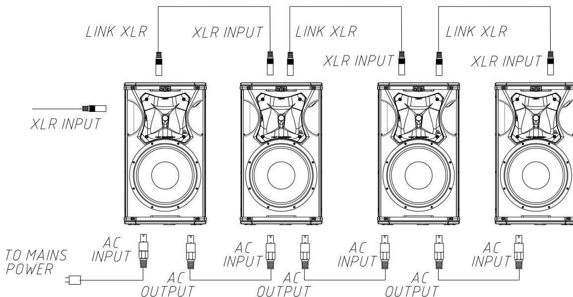
Fig. 3. Parallel connection for S12A7 (signal and mains)
