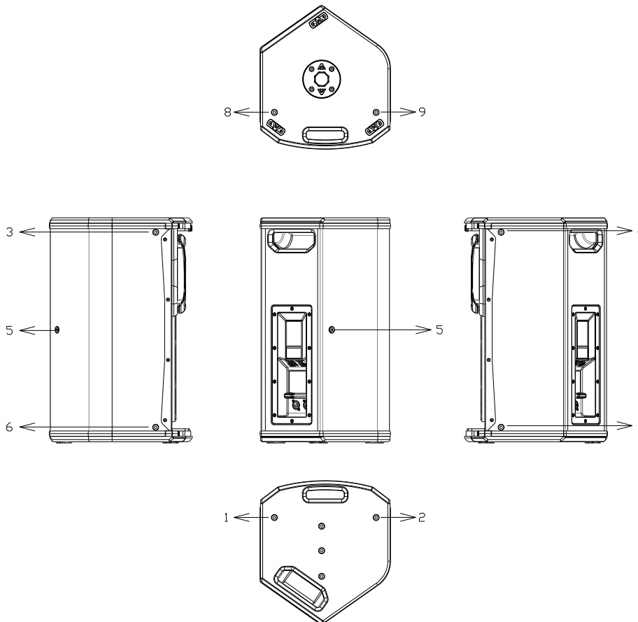
Fig. 16. S12A7 rigging points
