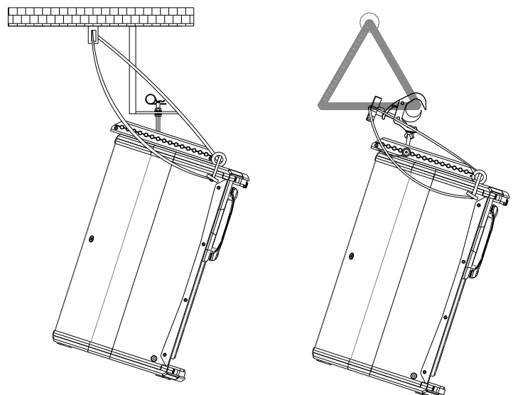
Fig. 14. RB-L and RB-L/GT flying bar for S12A7
