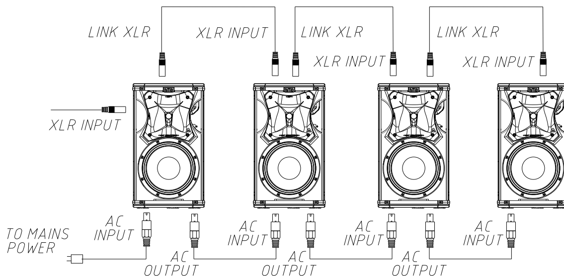
Fig. 3. Parallel connection for S10LT (signal and mains)
