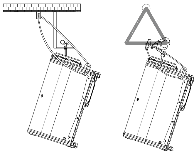
Fig. 16. RB-S and RB-S/GT flying bar for S10LT
