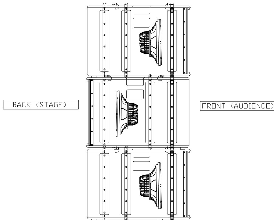
Fig.22. Cardioid configuration for X215W subwoofer
