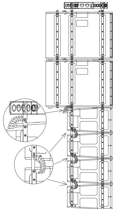
Fig.37. X215W Flying, three units in cardioid configuration
