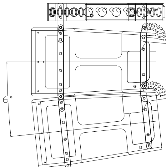
Fig.4. Tilt angle between cabinets (6° maximum)
