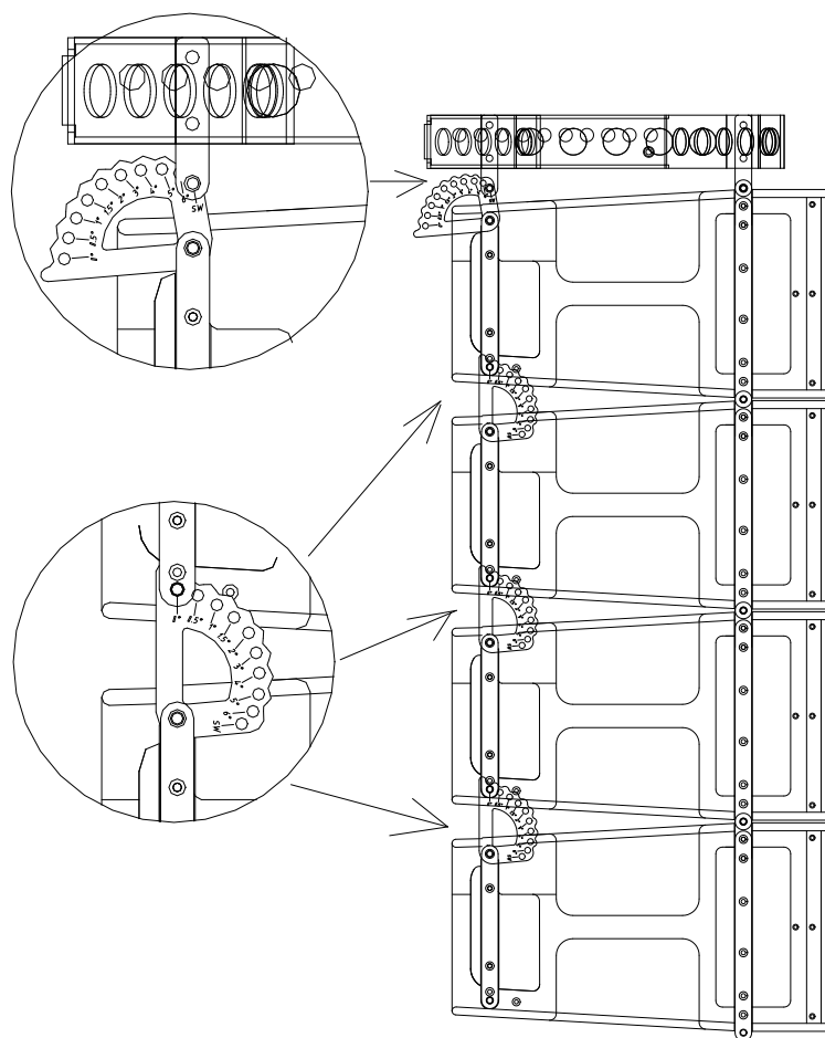
Fig.34. X210 Flying. Flat Line Array
