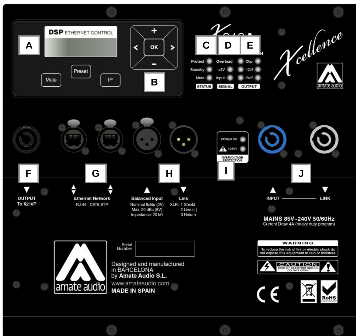
Fig.9. X210A control and connection panel
