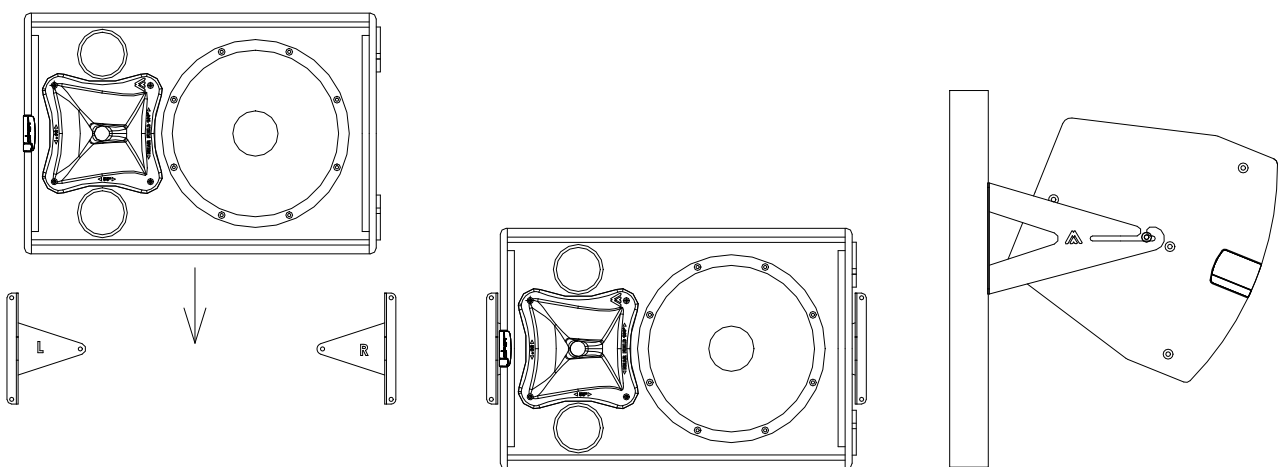
Fig.12. UB-L wall-stand
