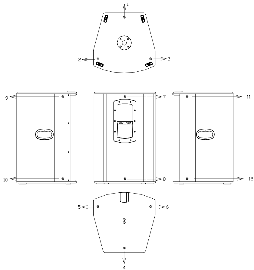
Fig.17. JK15NA rigging points
