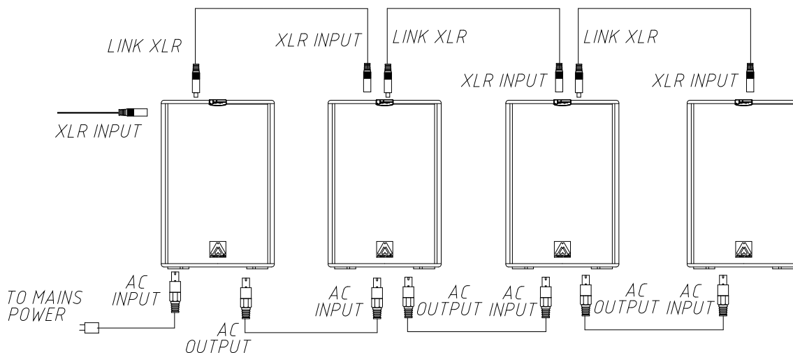
Fig.2. Parallel connection for Joker cabinets (signal and mains)
