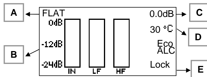
Fig. 27: Pantalla principal
