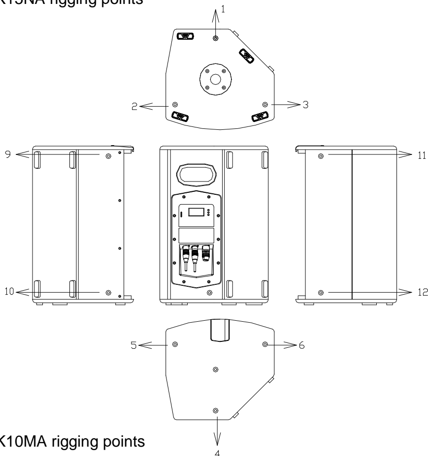
Fig.17. JK15NA rigging points
